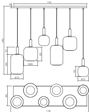
01-3215 Sand Black / Matt Gold E27, 6 x max. 23W
