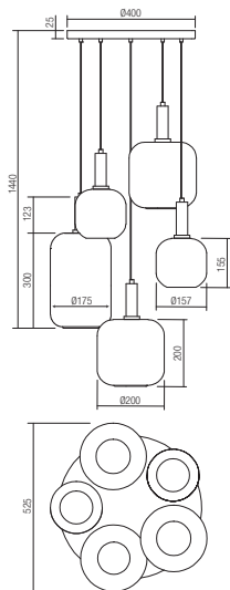
01-3214 Sand Black / Matt Gold E27, 5 x max. 23W
